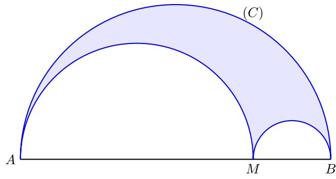
FIGURE 1 – Arbelos
