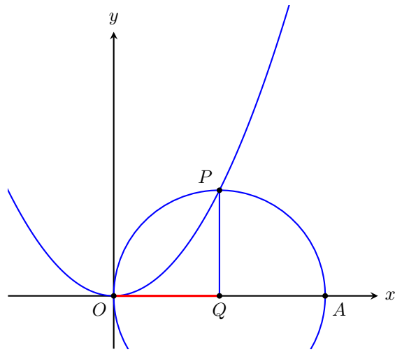
FIGURE 2 – Al_Khayam
