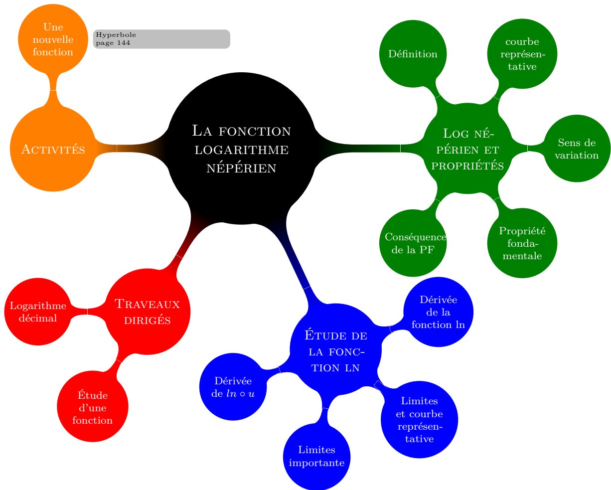
FIGURE 1 – MindMap Logarithme
